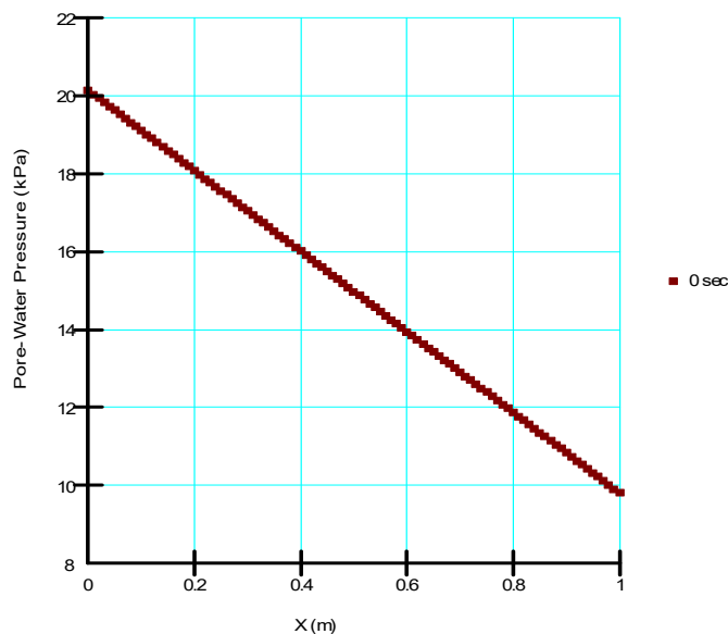
Figure 13. Pore-water pressure versus x-coordinate.
