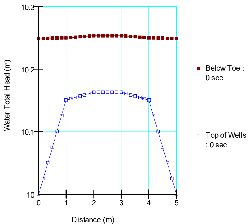
Figure 10. Head distribution between wells spaced 5 m apart
