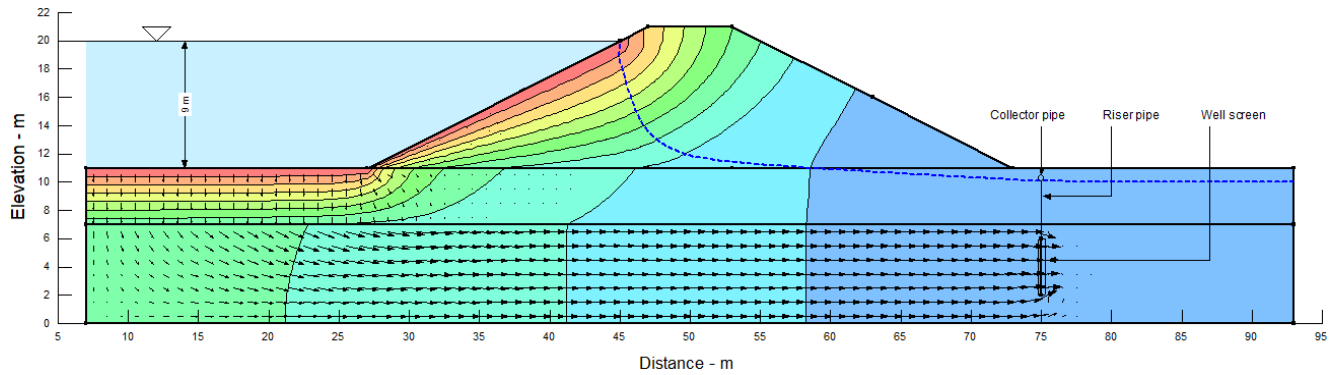
Figure 6. Phreatic surface, head contours and flow vectors given a 2D relief well (simulated trench)
