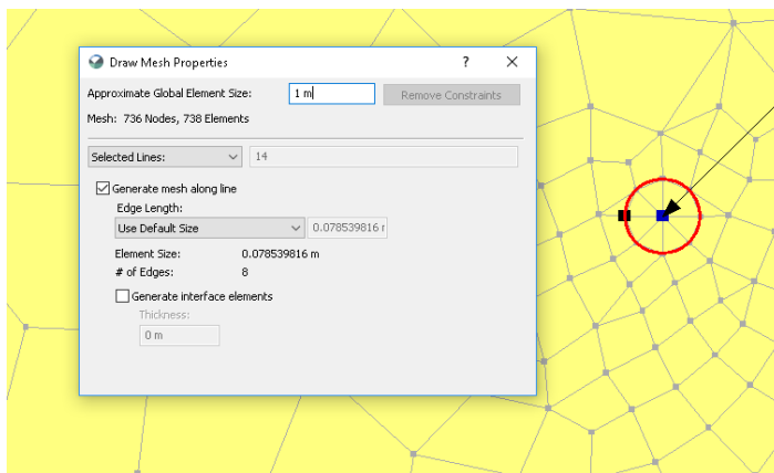
Figure 5. Mesh pattern around the circular opening.
