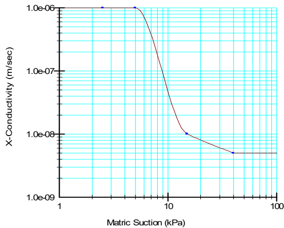
Figure 3. Hydraulic conductivity function of the soil material.
