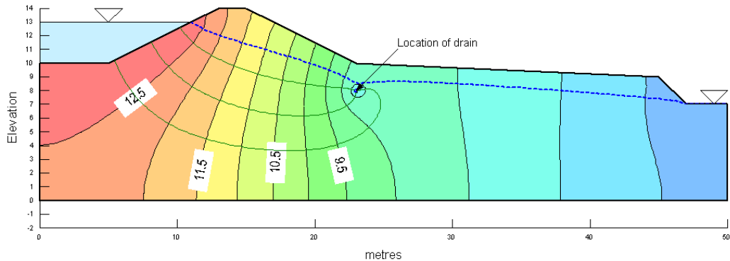
Figure 7. Resulting total head contours and flow paths with the drain present using the circular opening.
