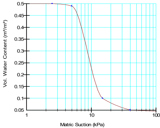
Figure 2. Volumetric water content function of the soil material.
