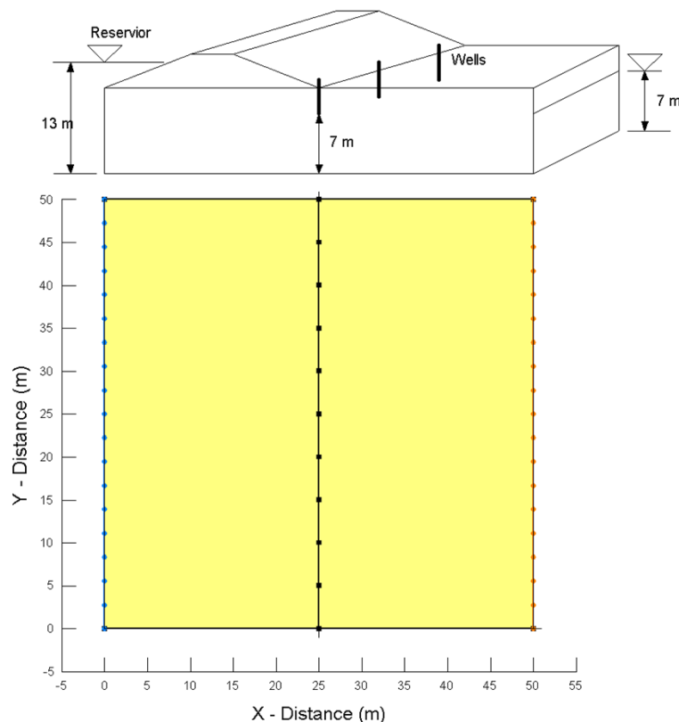
Figure 1. Problem schematic with SEEP/W plan view configuration.
