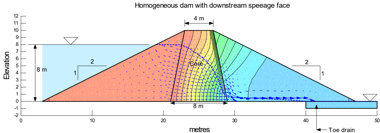
Figure 16. Flow regime with core K_{sat} reduced 100x.
