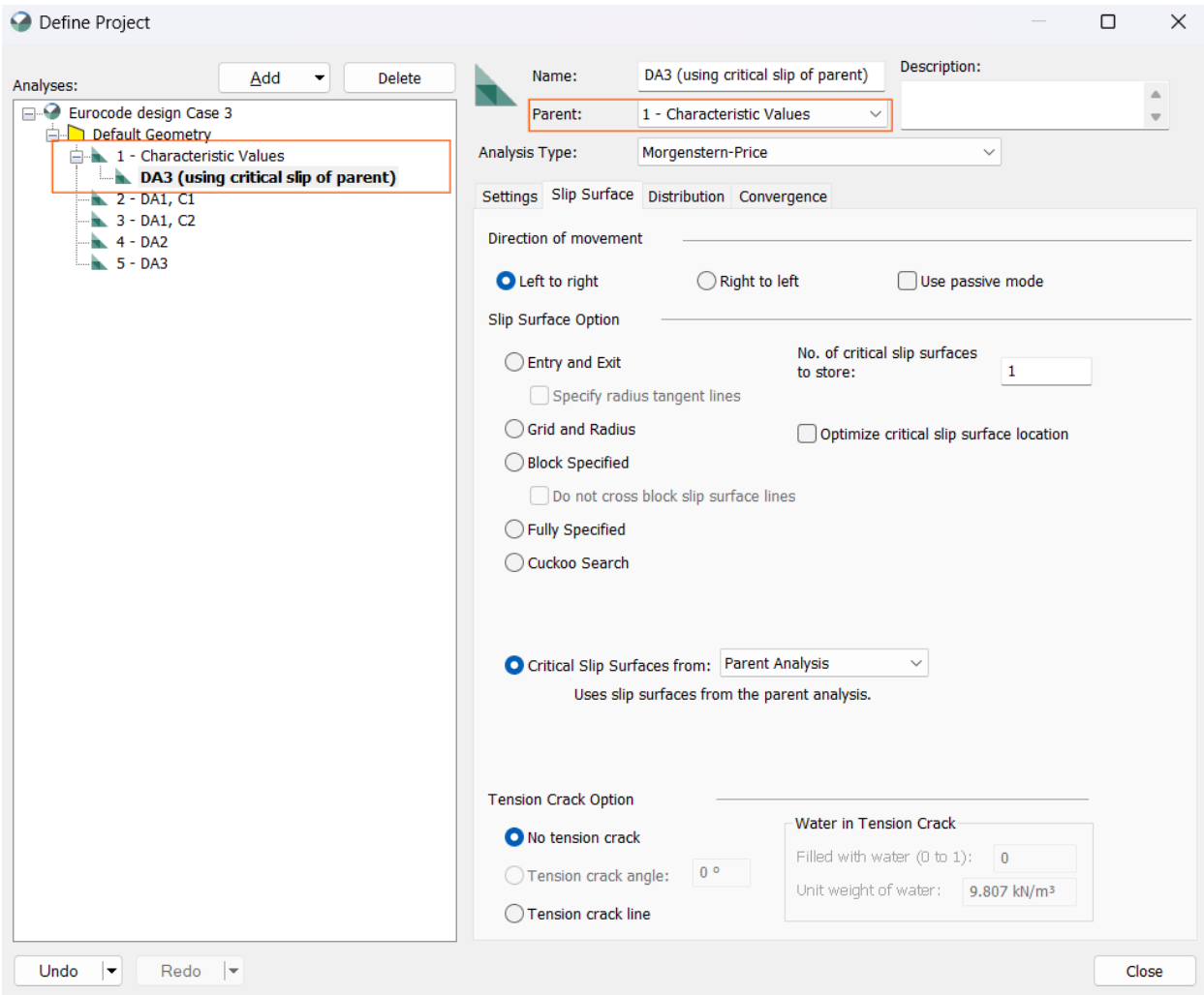
Figure 22. Analysis definition for completing a limit state design check on the critical slip surface located using characteristic values.
