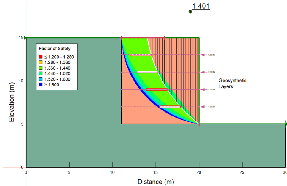
Figure 4. Stability results for the base case (Analysis 1) when the pullout resistance is a constant and the reinforcement is not factor of safety dependent.
