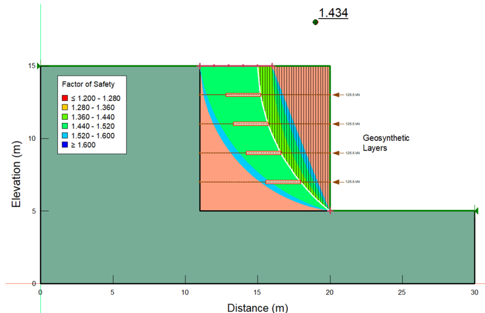
Figure 5. Stability results when the reinforcement load depends on the computed factor of safety (Analysis 2).
