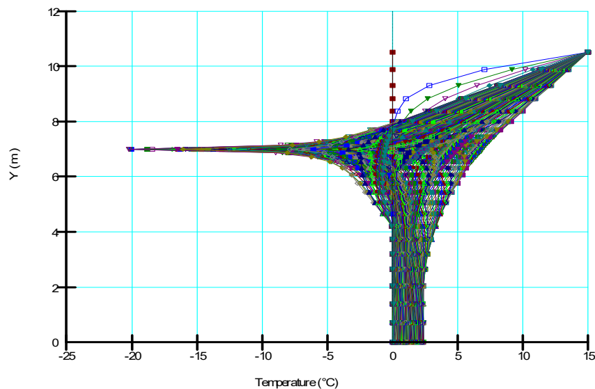
Figure 5. Temperature profile along left edge of model domain.
